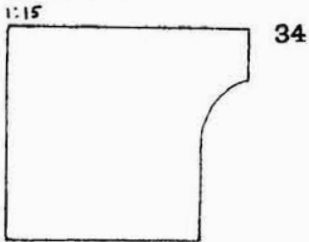
CAVETTO BRICK OF PYRAMID CORNICE
